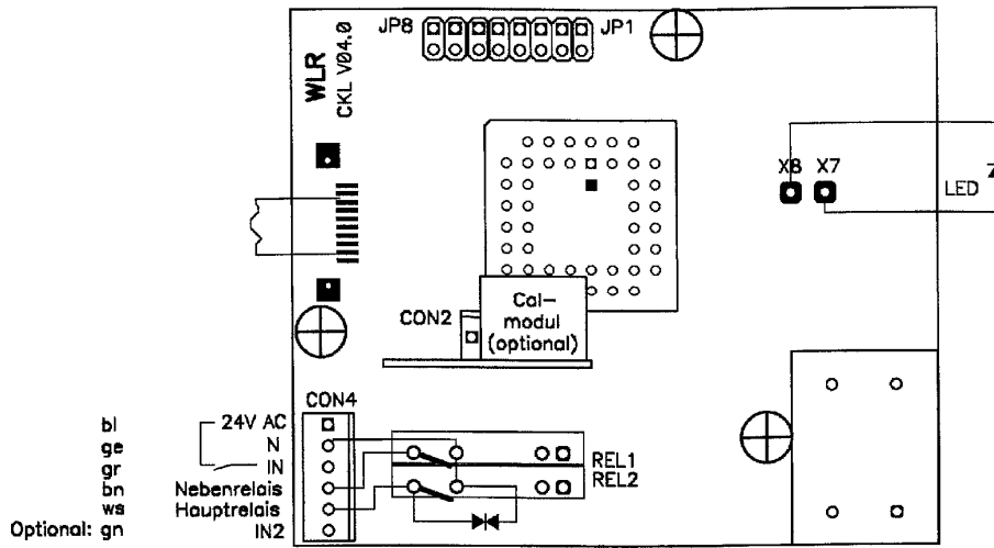
Chipkartenleser CKL V04.0
